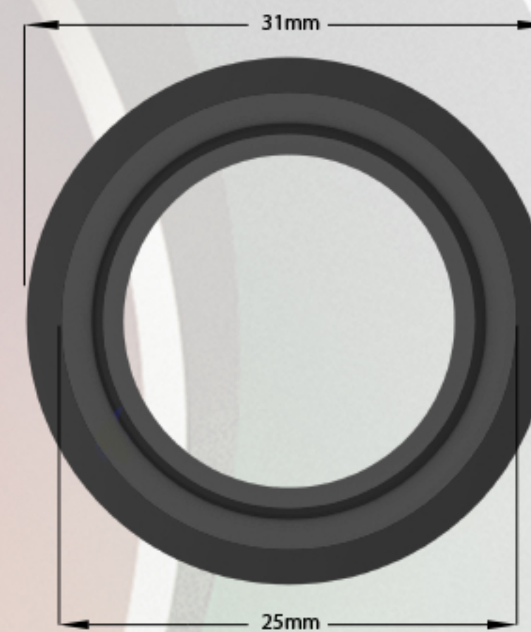
Jointing Socket Front Elevation
