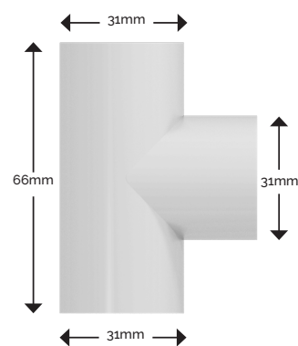
TEE FRONT ELEVATION
