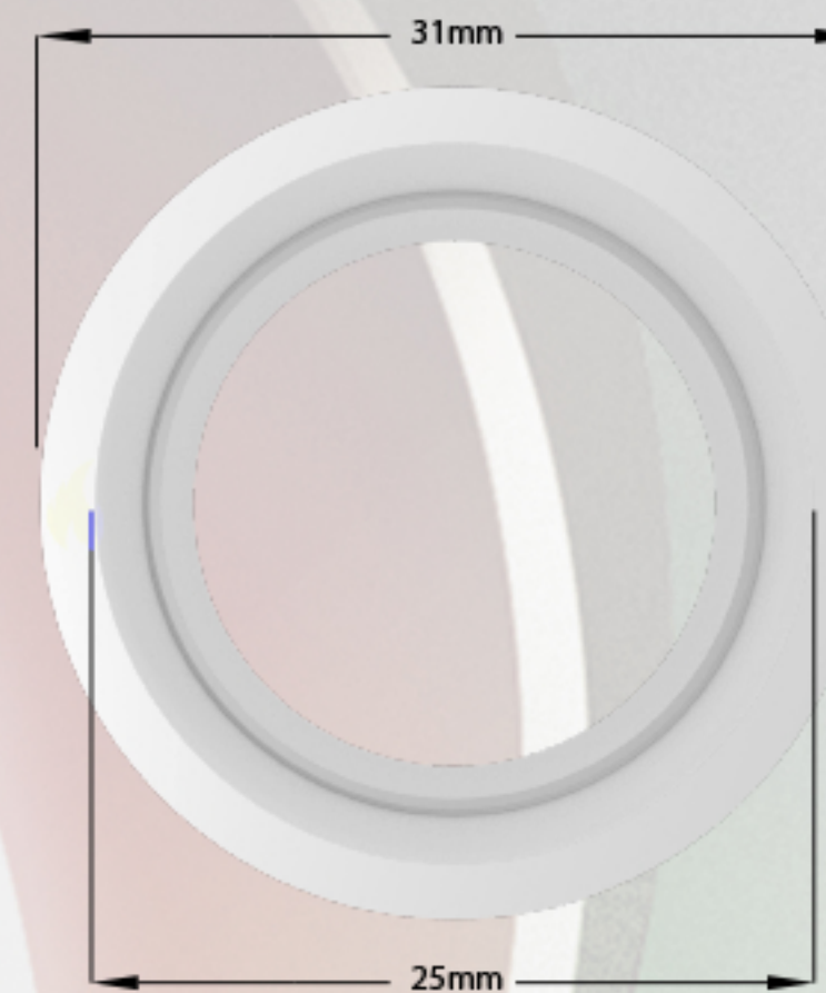
Jointing Socket Front Elevation
