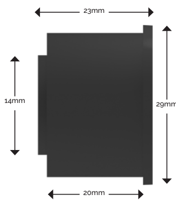
CAPILLARY ADAPTOR
