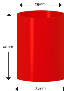
Joining Socket Side Elevation
