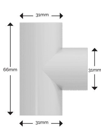
TEE ADAPTOR
