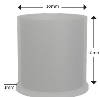
PROTECTION CAP
