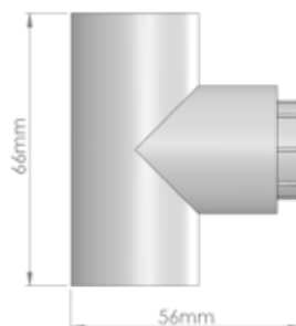
Side Elevation
