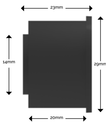
CAPILLARY ADAPTOR
