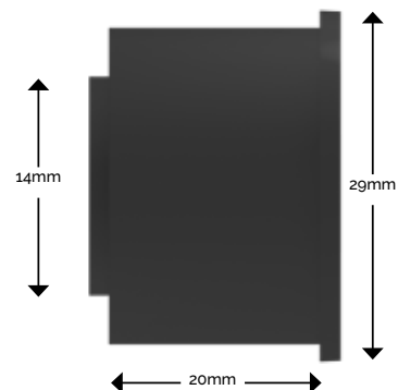
Capillary Adaptor
